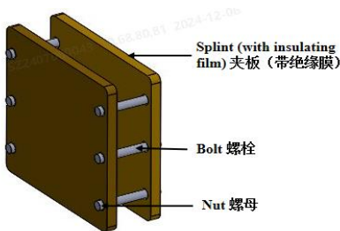
Fig. 1 Schematic diagram of cell clamp
