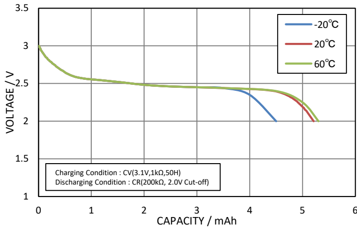
Discharging Characteristics
