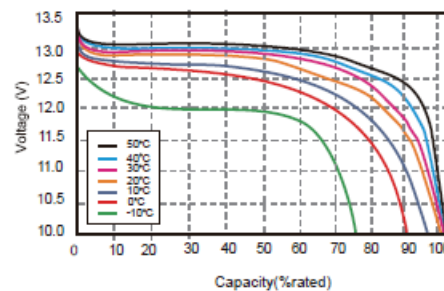
DISCHARGE CAPACITY at VARIOUS TEMPERATURES DISCHARGE @0.5C
