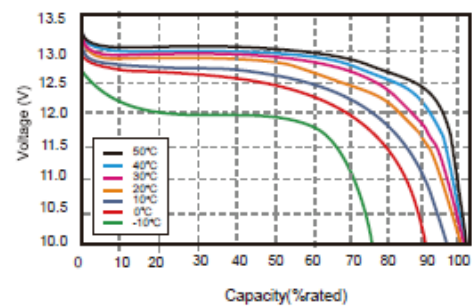
DISCHARGE CAPACITY at VARIOUS TEMPERATURES DISCHARGE @1C
