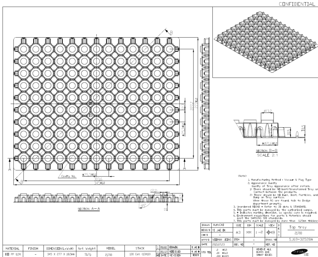
Fig. 2-3. Upper tray drawing.
